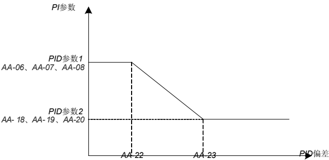
图5-24.PID参数切换
